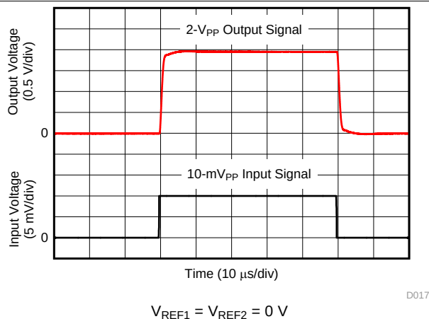
Figure 20. Step Response (10-mV pp Input Step)
