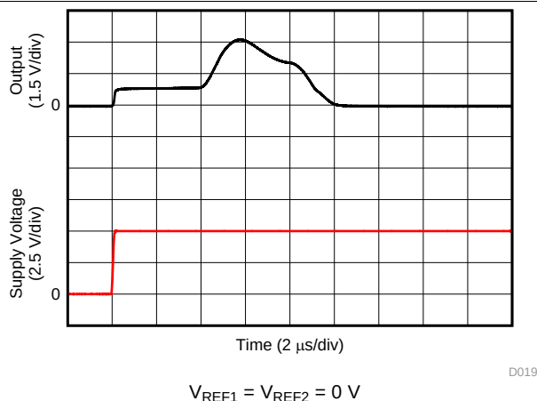
Figure 22. Start-Up Response
