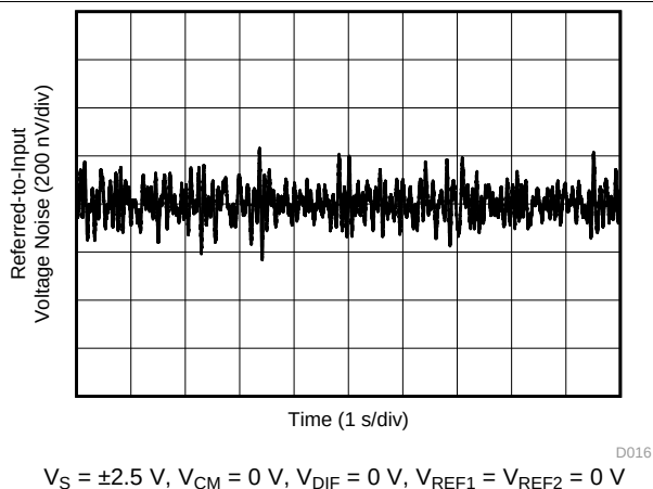
Figure 19. 0.1-Hz to 10-Hz Voltage Noise (Input Referred)
